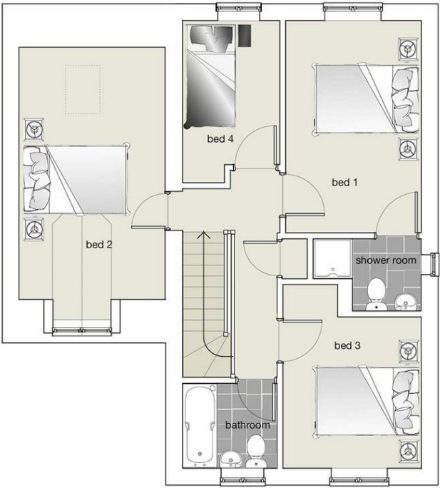
First Floor Plan bedroom 1 4.43 x 2.78 bedroom 2 4.13 x 2.88 (@ 1.5m headroom) bedroom 3 3.08 x 2.82 bedroom 4 3.04 x 2.00
